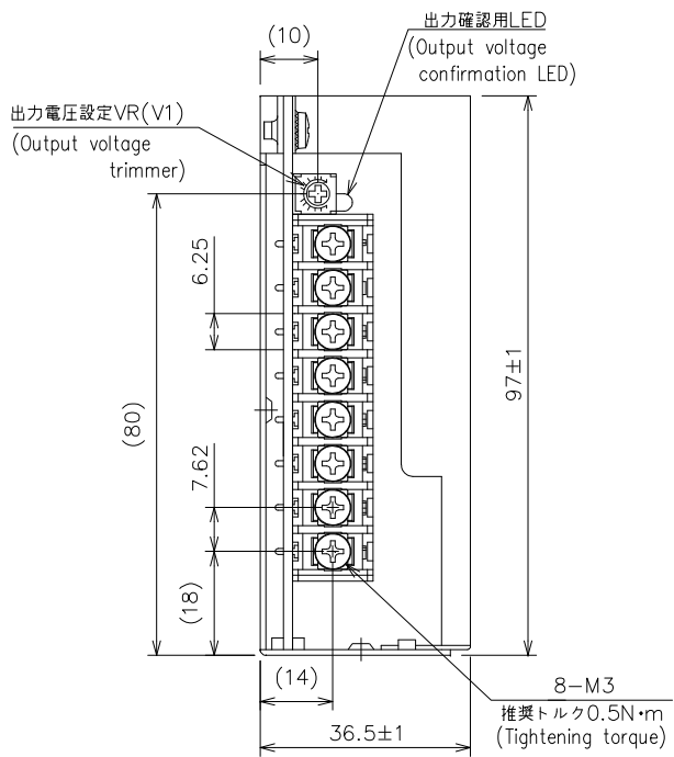
・端子台接続表 Connection of terminal block
