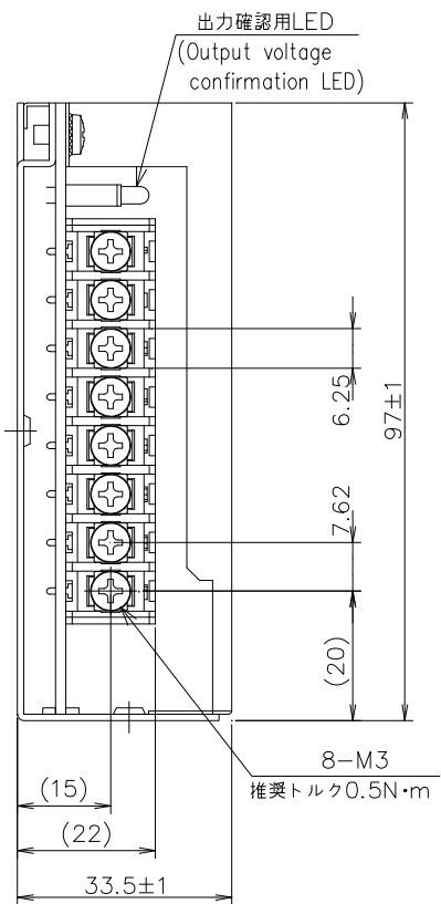
・端子台接続表 Connection of terminal block
