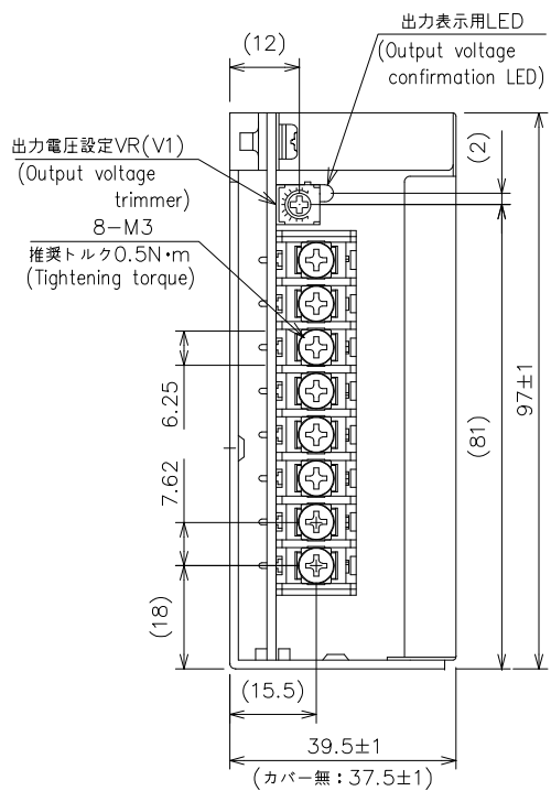
・端子台接続表 Connection of terminal block
