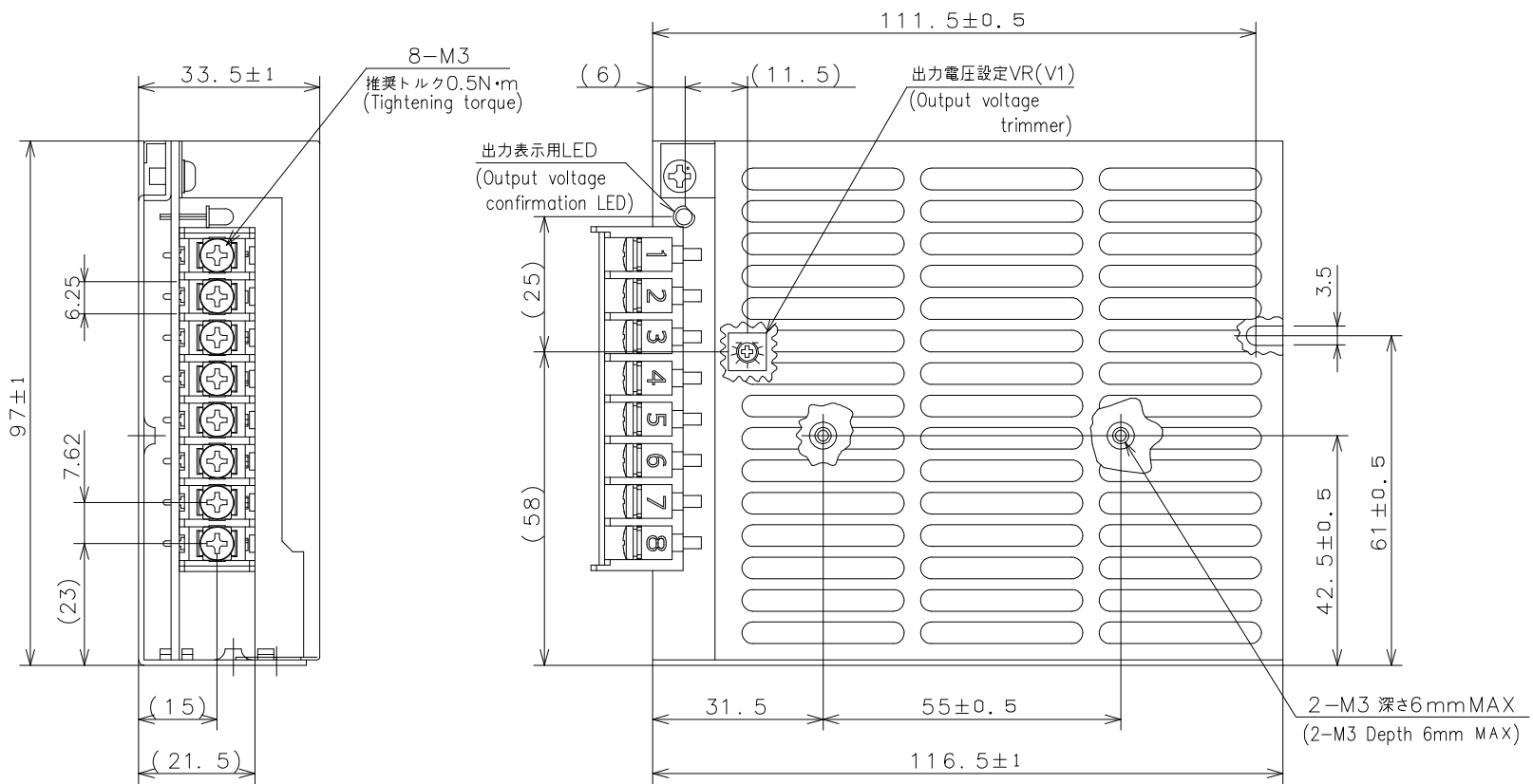
・端子台接続表 Connection of terminal block
