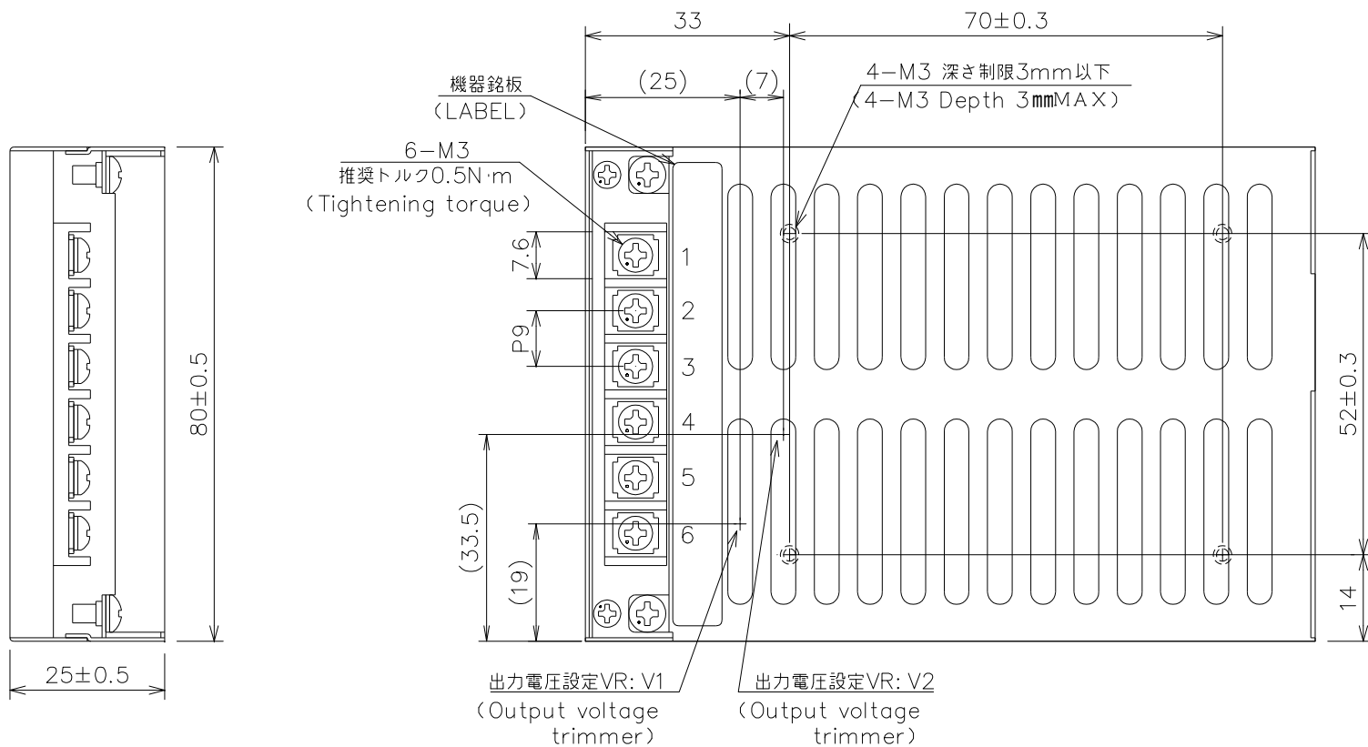
・端子台接続表 Connection of terminal block
