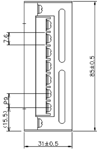
・端子台接続表 (Connection of terminal block.)
