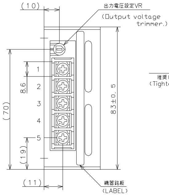
・端子台接続表 (Connection of terminal block.)
