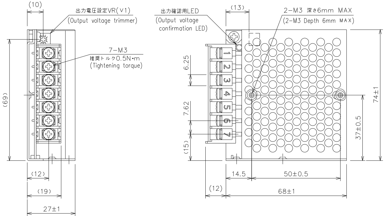
・端子台接続表 (Connection of terminal block)
