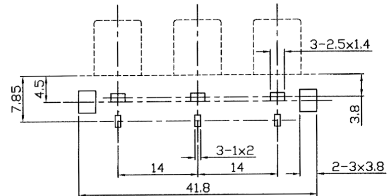
PC BOARD HOLE LAYOUT GEN TOLS: \pm 0.1\text{mm} (VIEW FROM DIRECTION OF INSERTION TO PCB)
