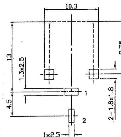
PC BOARD HOLE LAYOUT
