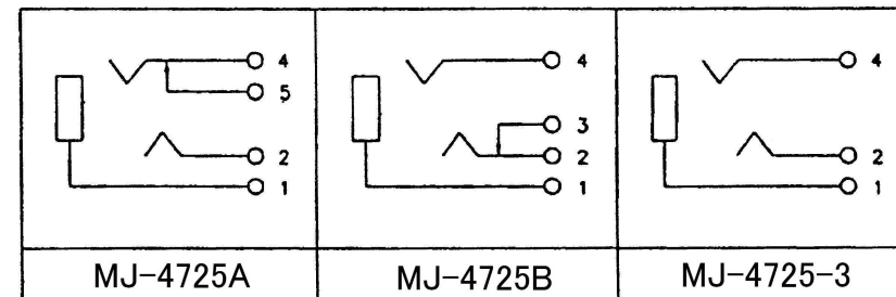
ALTERNATIVE MODELS CIRCUITRY
