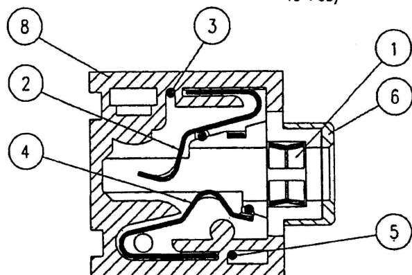
SECTION AA 4/1 mm
