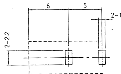
PC BOARD HOLE LAYOUT (UPPER VIEW FROM THE DIRECTION OF INSERTION TO PCB.)
