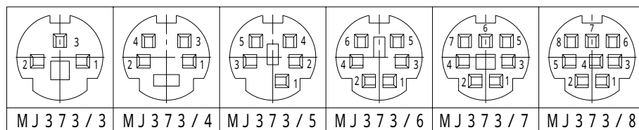
CONTACT CONFIGURATIONS
