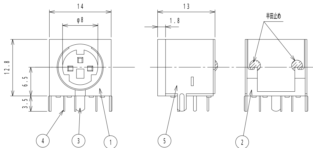
CONTACT CONFIGURATIONS
