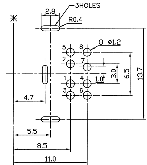
T:1.6 Dimensions of PC board holes Tolerance : \pm 0.05 (Printed-top view)
