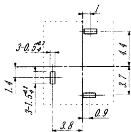
P.C. Hole Layout (Mounting view) for reference only
