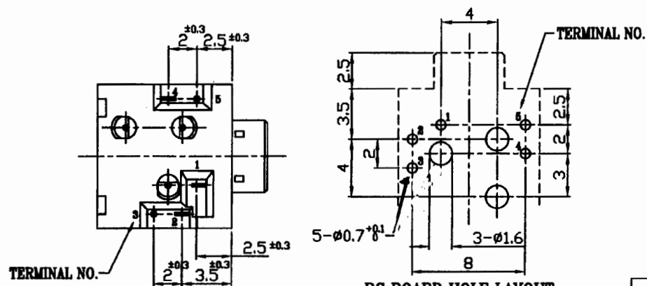
PC BOARD HOLE LAYOUT (VIEW FROM DIRECTION OF INSERTION TO PCB)
