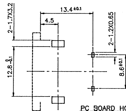
PC BOARD HOLE LAYOUT
