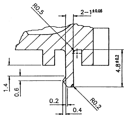
DETAIL OF P 4/1 mm
