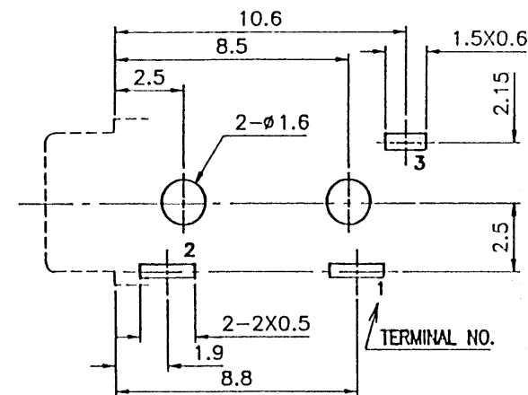
PC BOARD HOLE LAYOUT (VIEW FROM DIRECTION OF INSERTION TO PCB)
