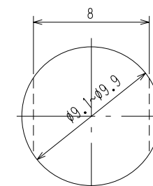
取付板板厚 Thickness of mounting board t=1.0~1.8
