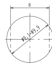
取付板板厚 Thickness of mounting board t=1.0~1.8
