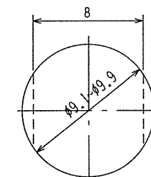
取付板板厚 Thickness of mounting board t=1.0~1.8
