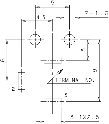
PC BOARD HOLE LAYOUT (VIEW FROM DIRECTION OF INSERTION TO PCB)
