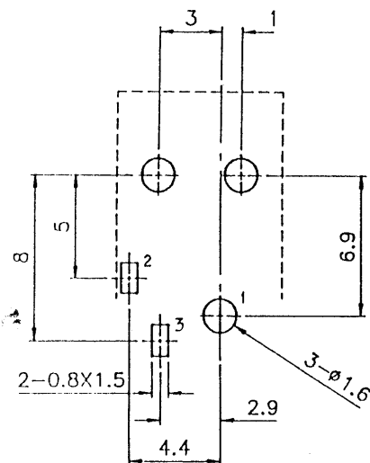
PC BOARD HOLE LAYOUT (VIEW FROM DIRECTION OF INSERTION TO PCB)
